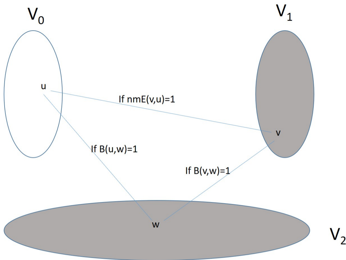
Figure 2. Illustrating the construction of Theorem 8.7.
