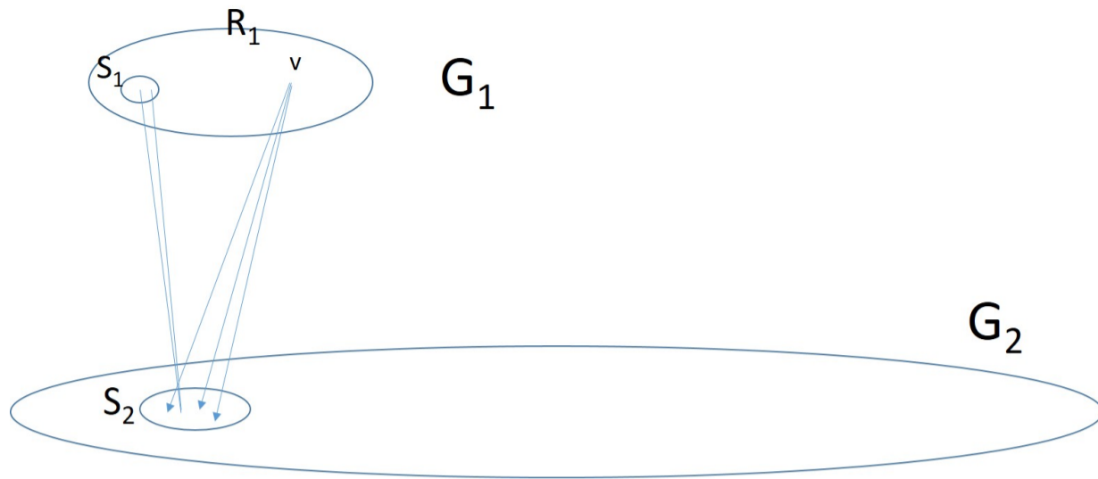
Figure 3. The construction of Theorem 8.10.
