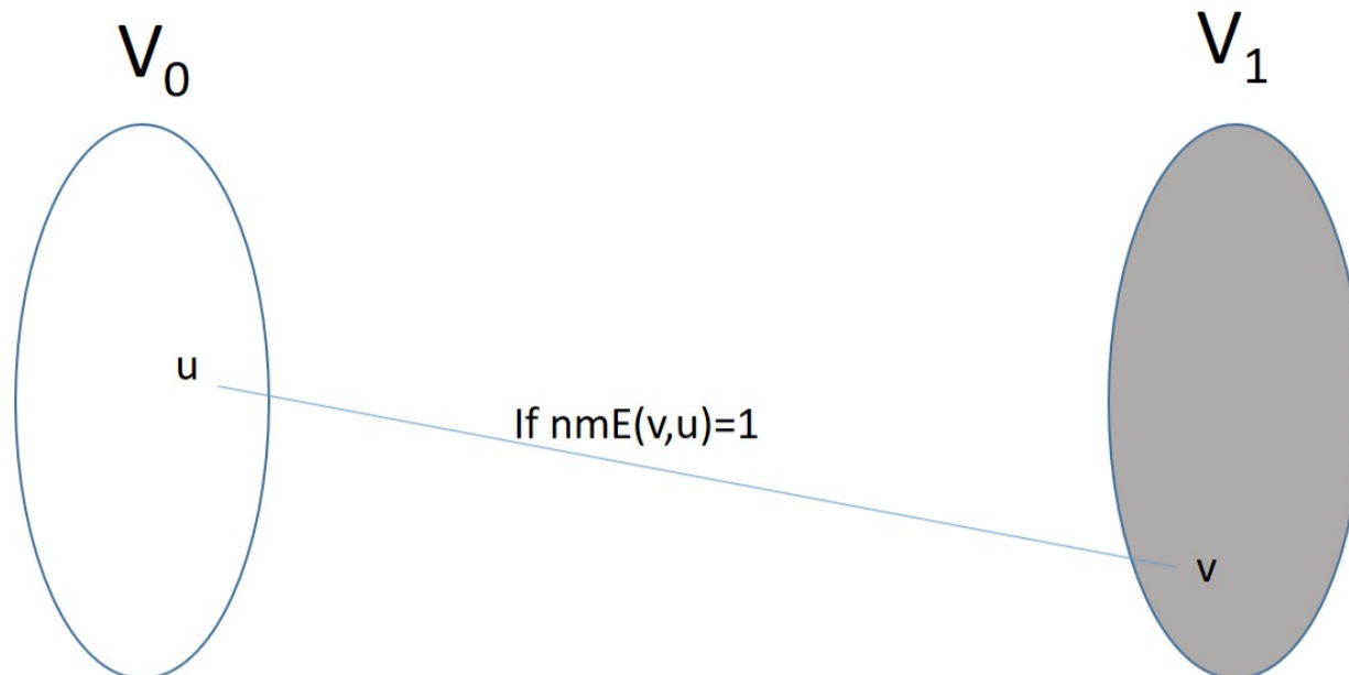
Figure 1. Illustrating the construction of Theorem 8.3.
